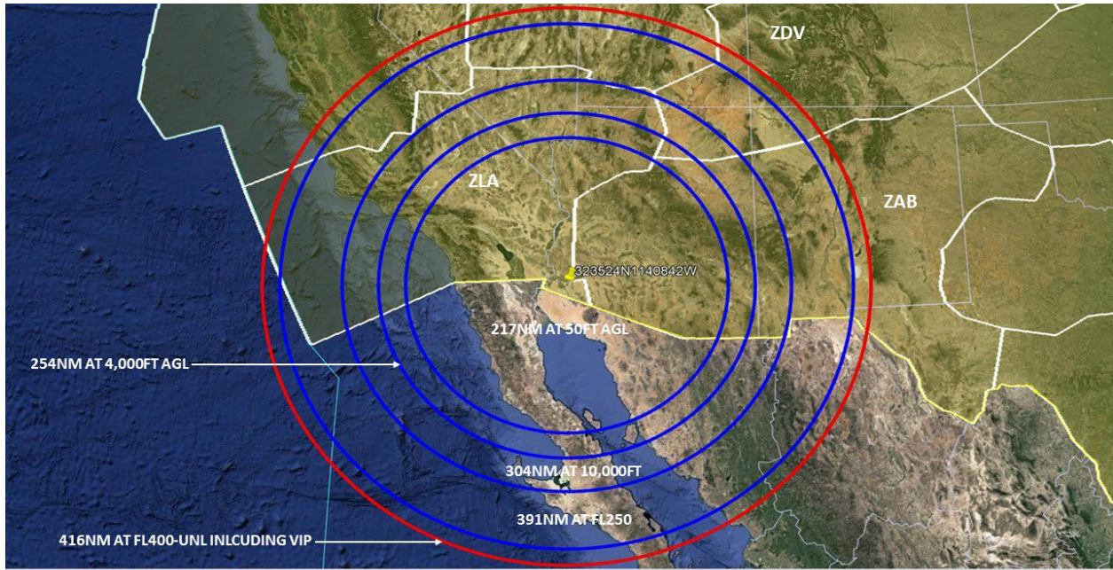
MCASAZ GPS 24-02 (Revision 1) GPS INTERFERENCE TESTING
