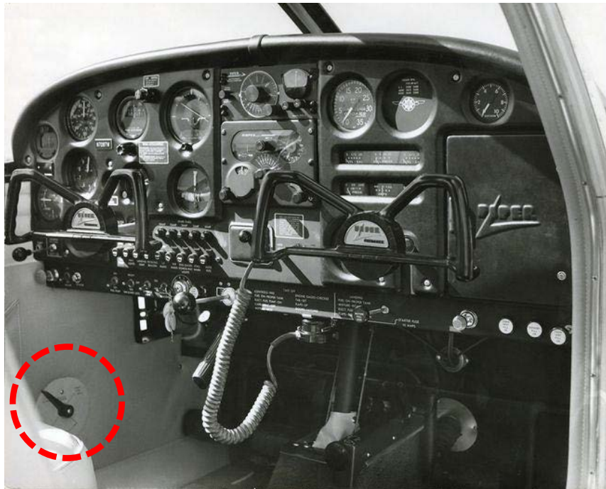
Figure 1: PA-28 Cockpit View Showing location of Generation 1 Fuel Selector
