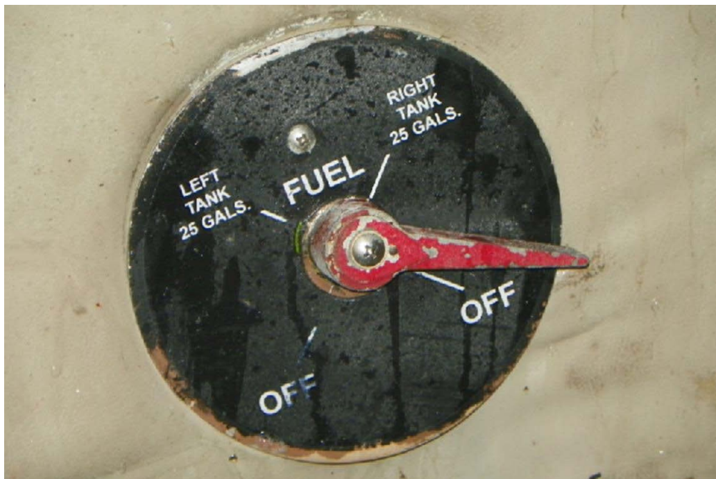
Figure 2: Generation 1 Fuel Selector
