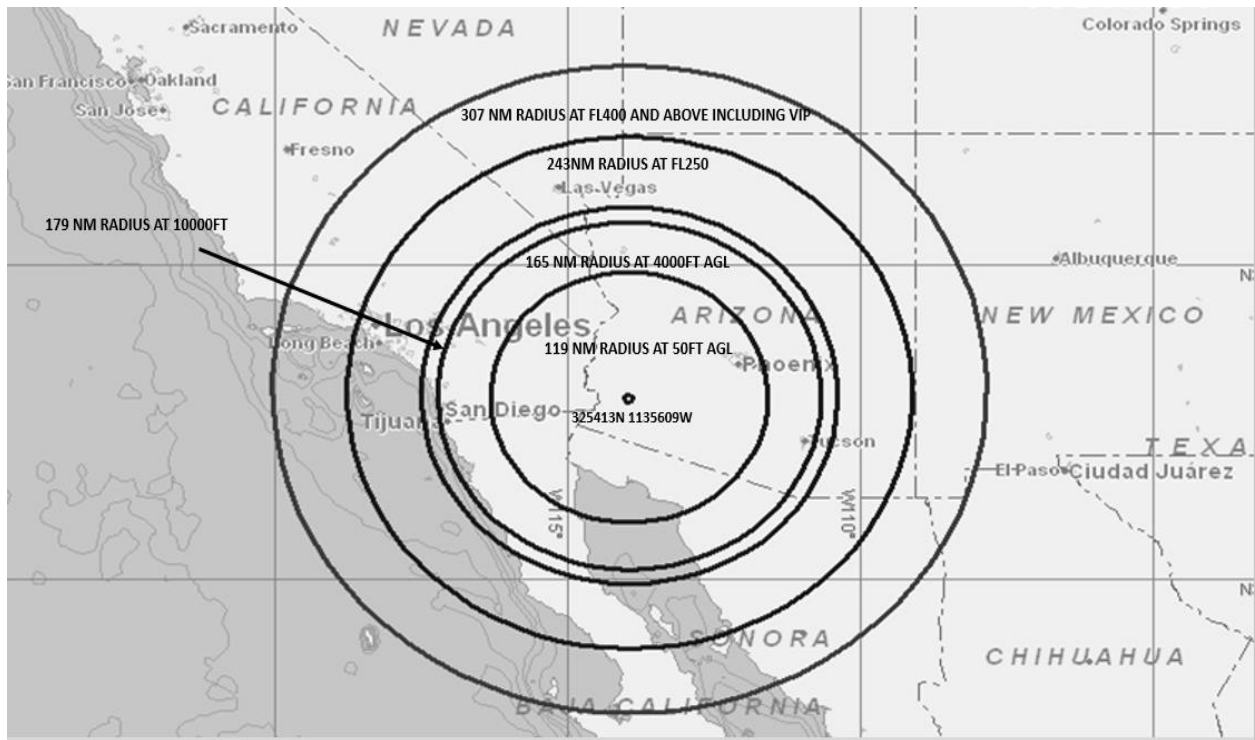
YPG 18-10 GPS INTERFERENCE TESTING
