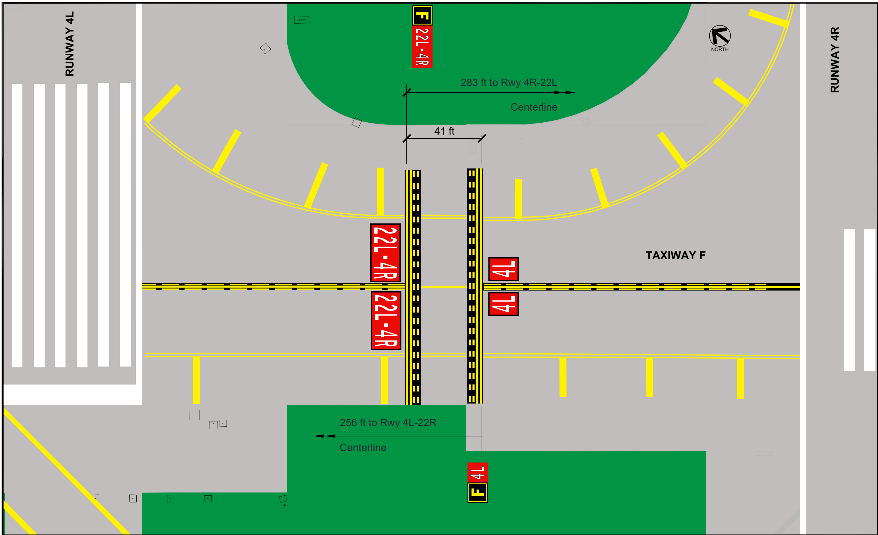
HNL RWY 4L/4R - TXY F Existing Configuration
