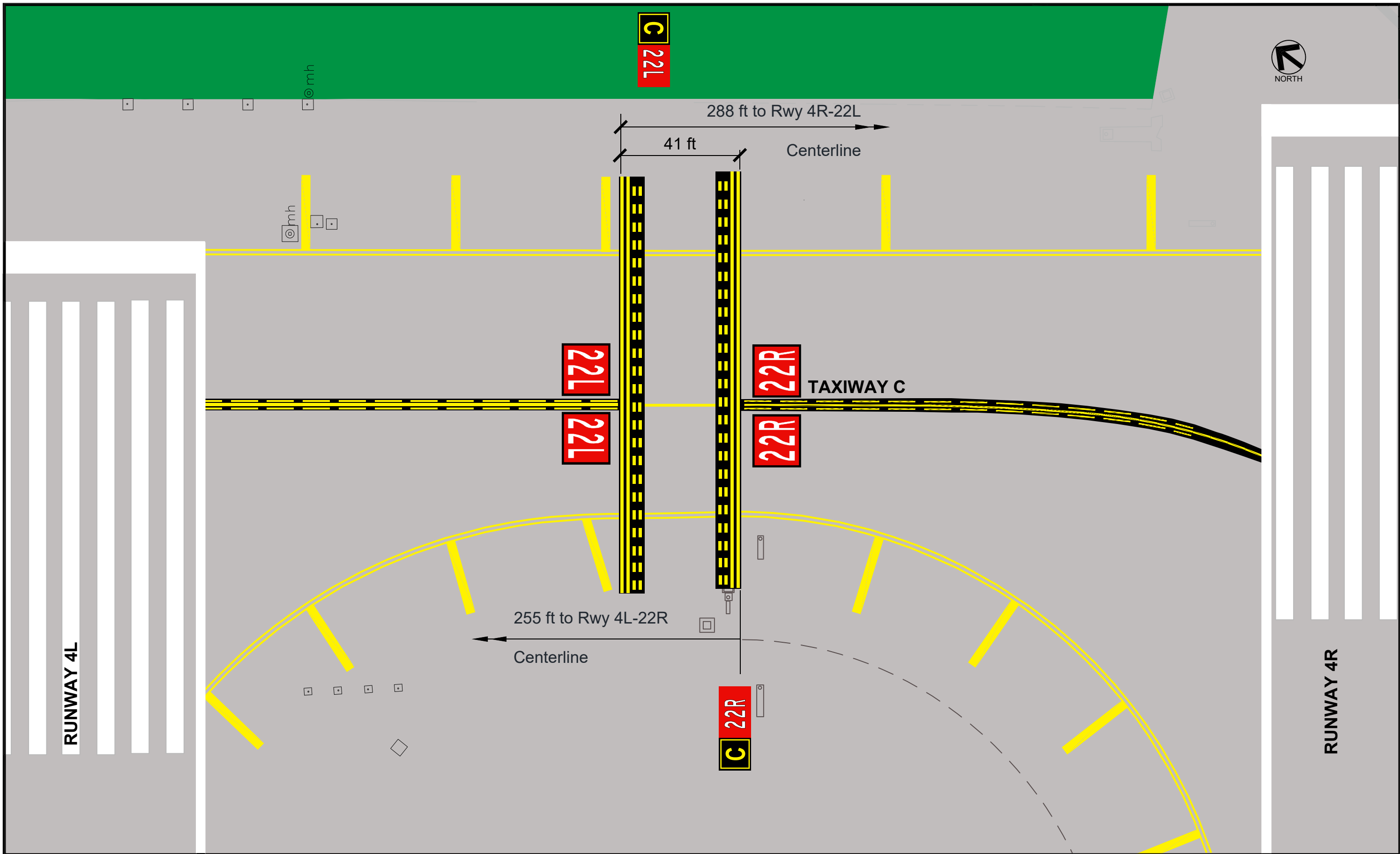
HNL RWY 4L/4R - TXY C Existing Configuration
