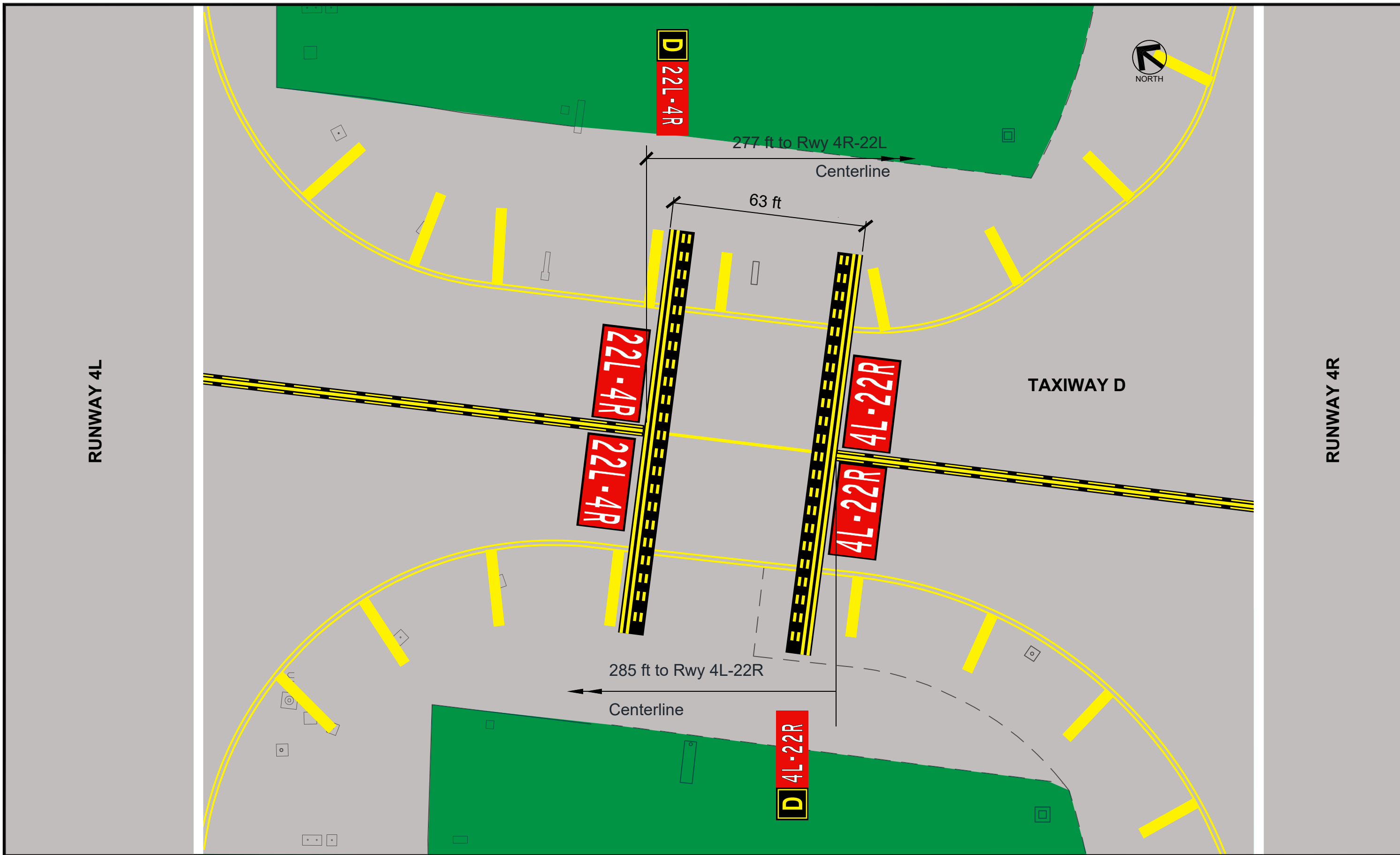
HNL RWY 4L/4R - TXY D Existing Configuration
