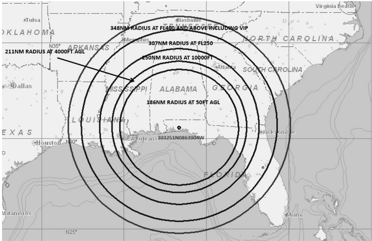
GAFC 17-10 GPS INTERFERENCE TESTING
