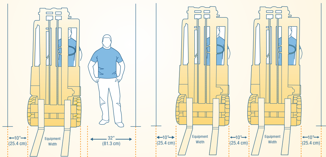
Figure 4-3: Aisle and Corridor width when equipment maneuvering is required
