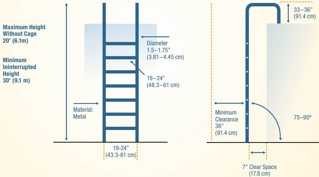
Figure 4-11. Recommended dimensions for fixed ladders
