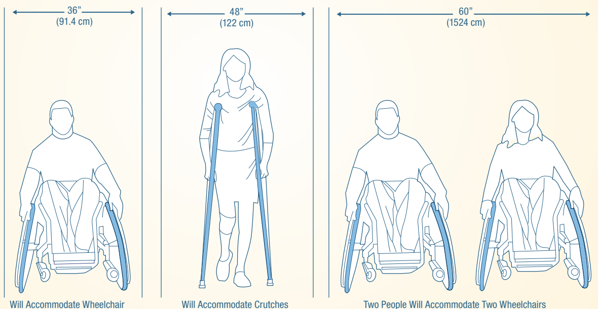
Figure 4-2: Recommended width for aisles and corridors
