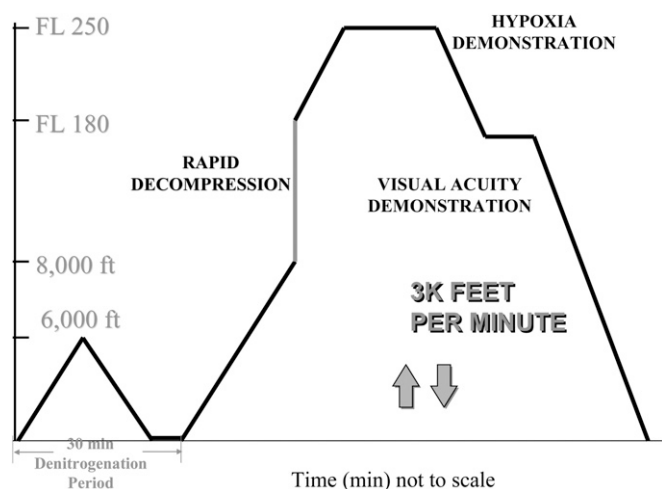
Fig. 1. Altitude chamber flight profile.
