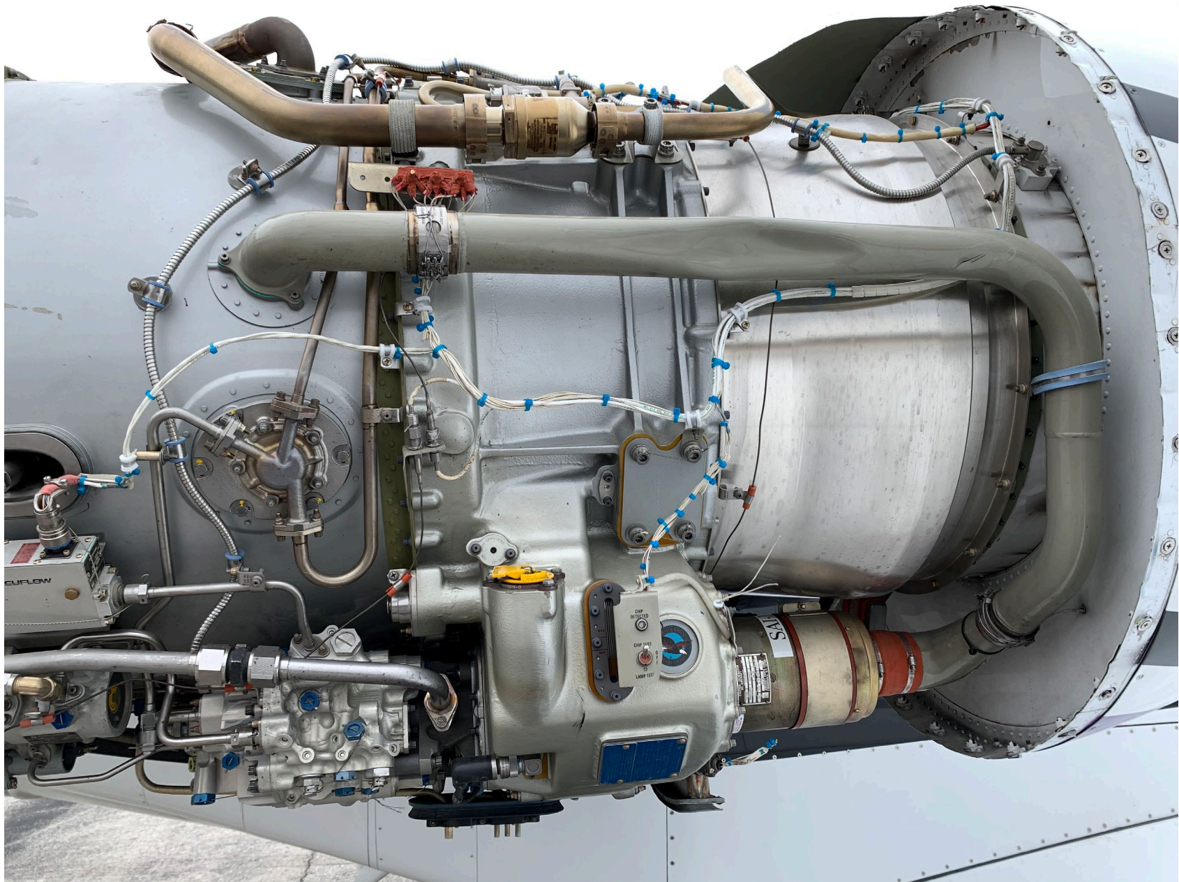
Photo 6 – View of the fractured upper and missing lower right side engine cowlings (courtesy of the Federal Aviation Administration).
