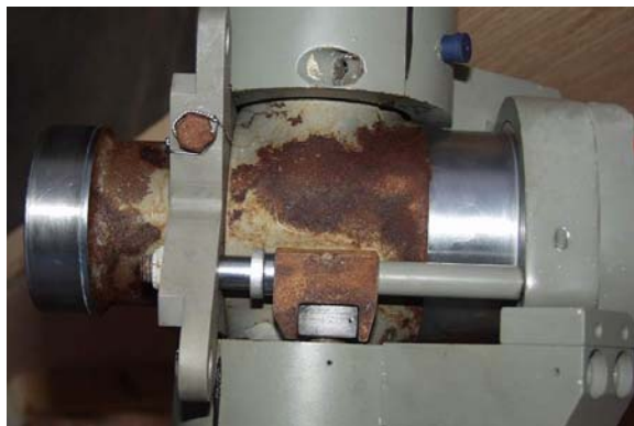
FIGURE 1-1. Hub Surface Corrosion
