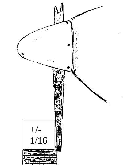
FIGURE 6. PROPELLER TRACKING
