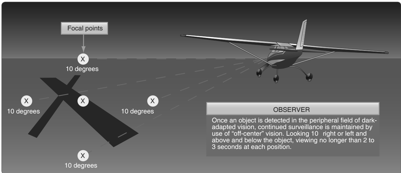
Figure 17-19. Off-center viewing.
