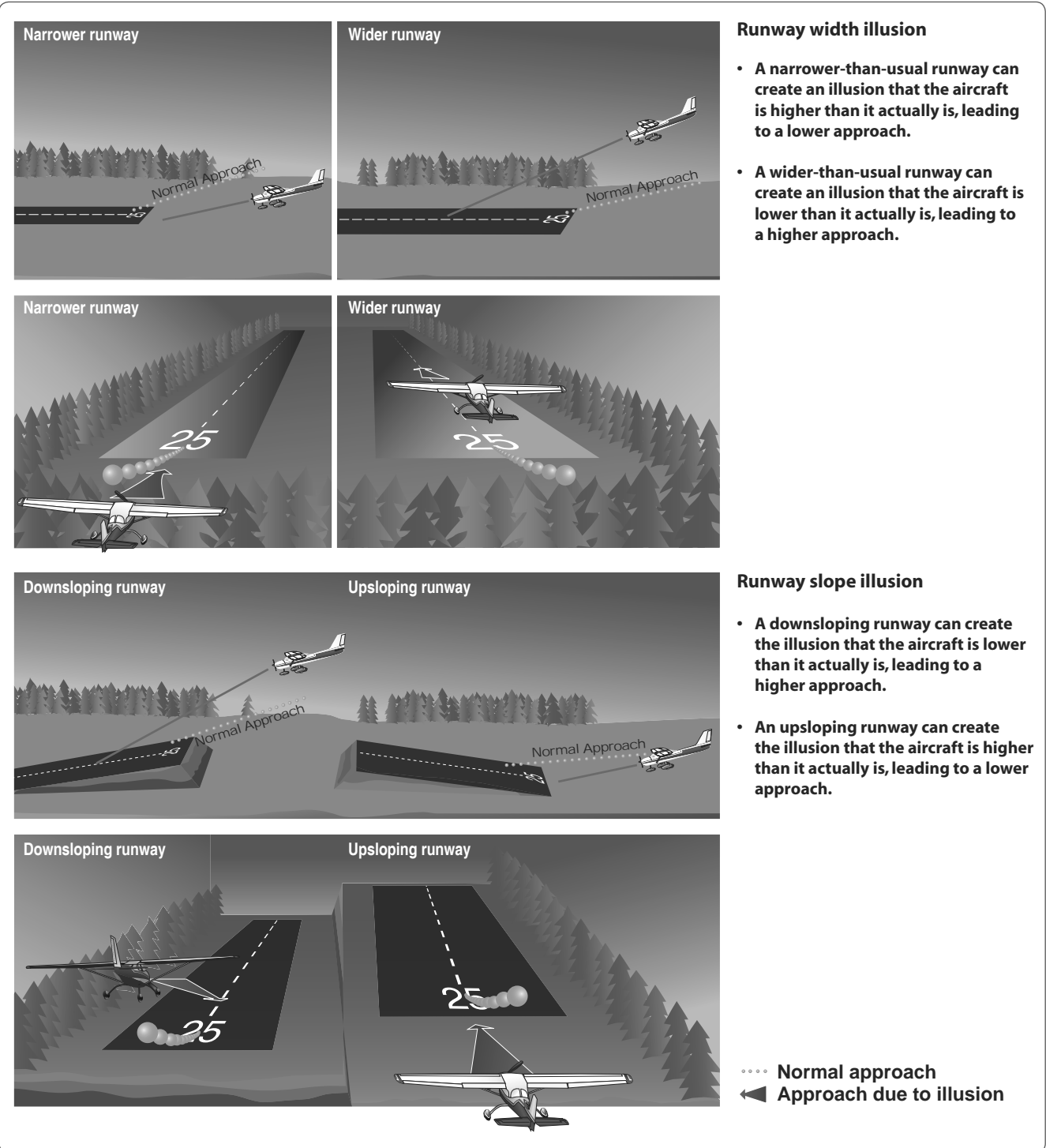
Figure 17-7. Runway illusions.
