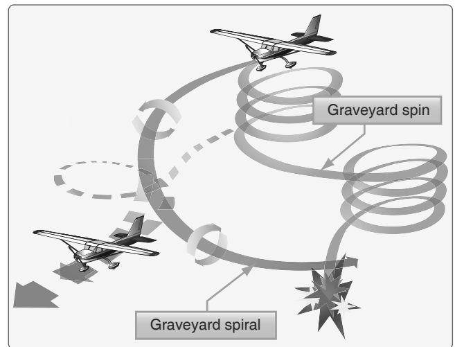
Figure 17-5. Graveyard spiral.
