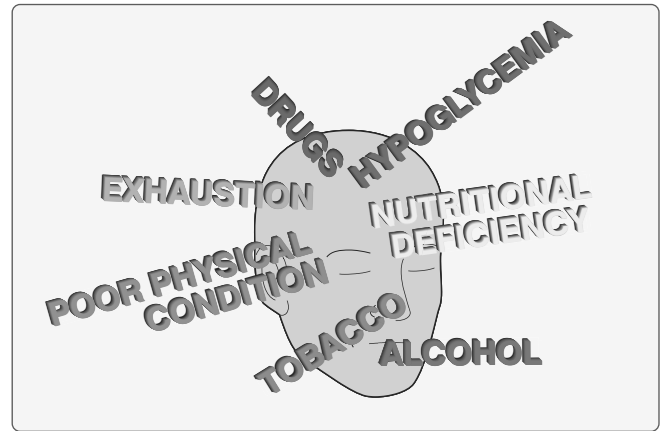
Figure 17-20. Self-imposed stress.
