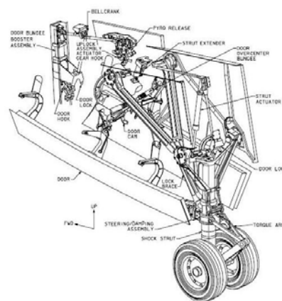
Nose Landing Gear Deployed
