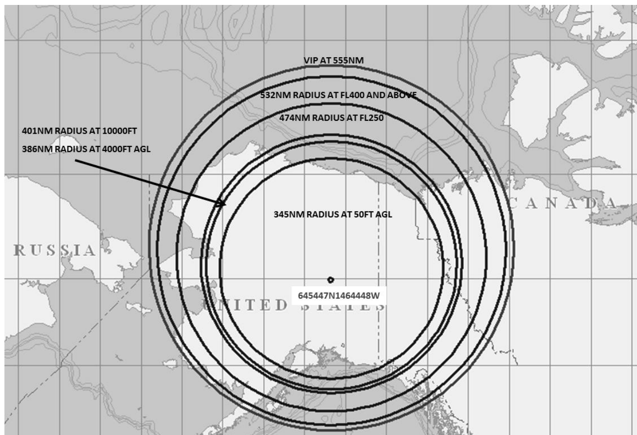
JFAK 17-01 GPS INTERFERENCE TESTING
